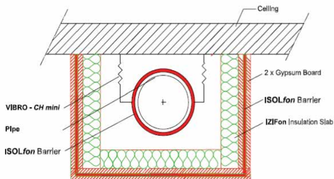
Typical Application in waste pipe noise insulation
