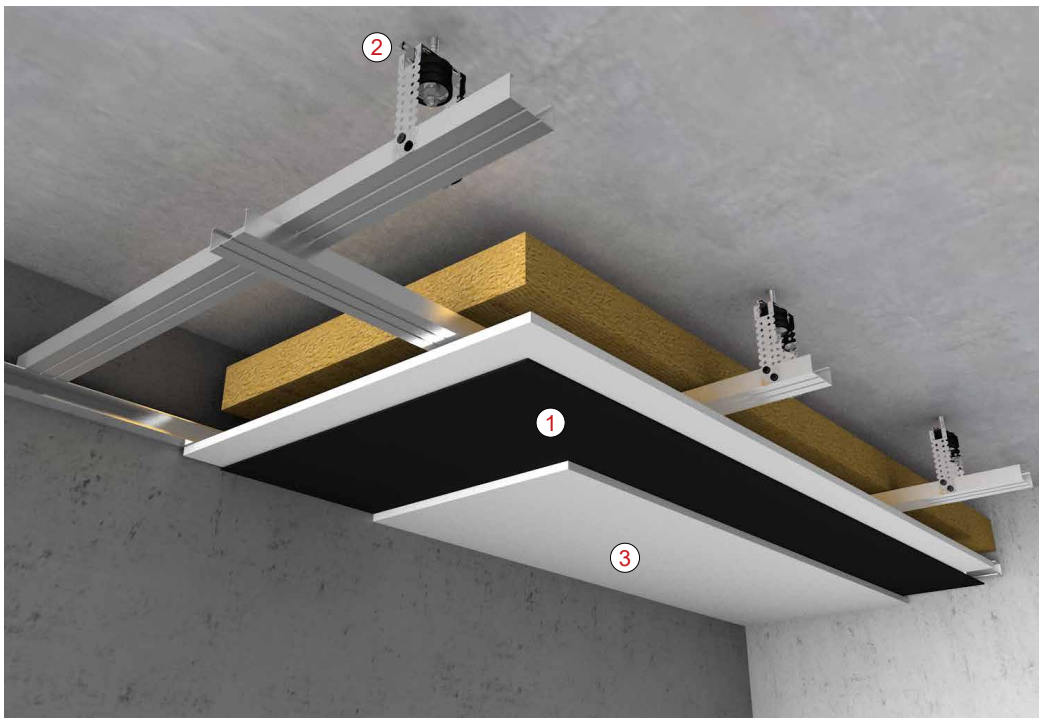
Sound Insulation for floating ceiling
